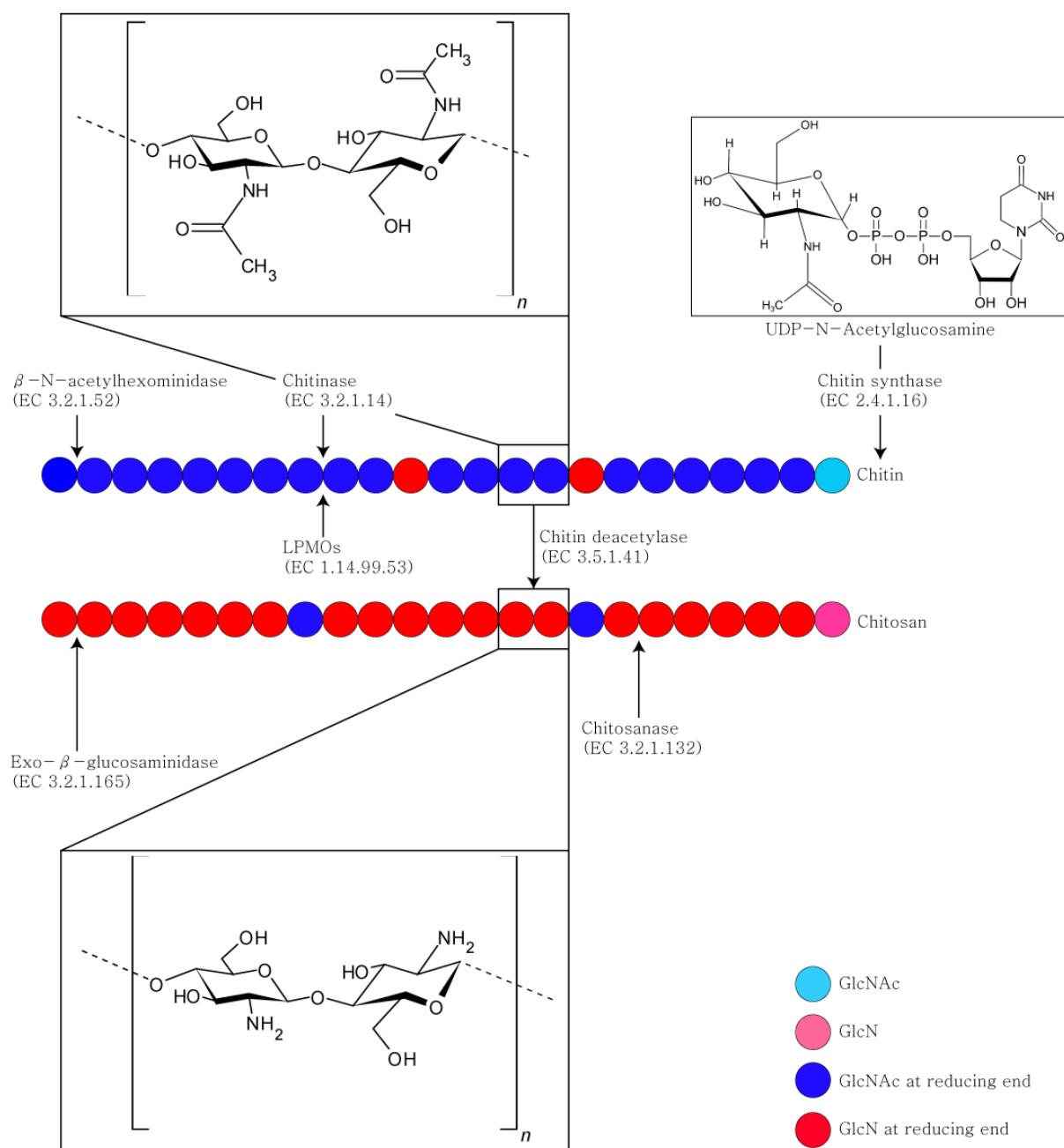
Fig. S1. Chemical structure of chitin, chitosan, and chitin-related enzymes. Chitin and chitosan are composed of two units in different proportions. Seven representative chitin-related enzymes, classified in the CAZy database (Lombard et al. , 2014), are shown.
